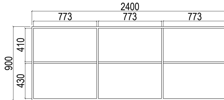
CUPBOARD DETAIL VIEW
